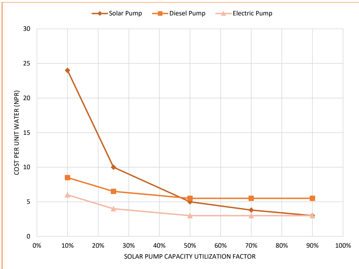
Figure 10: Cost per unit water in different pumping technologies in Nepal Source: (Renewable World, 2018) |
